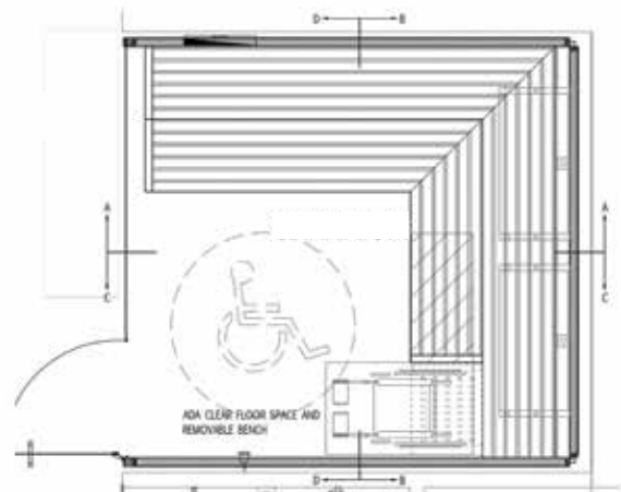
Illustration of a sauna providing correct wheelchair access and parking.
