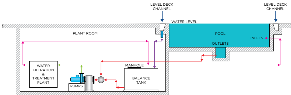
Option 2: Pool Water Treatment Plant & Balance Tank on Level Below
