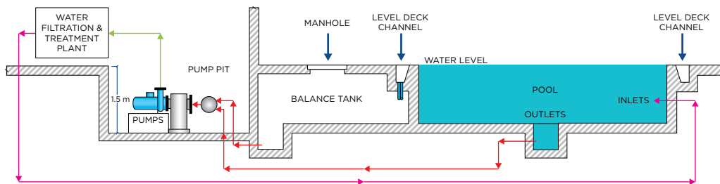
Option 1: Pool Water Treatment Plant on Same Level as Pool
